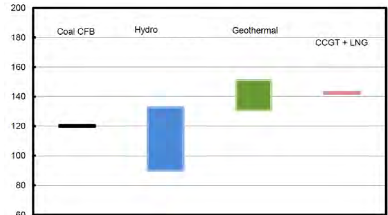
Levelised cost of electricity ($/MWh)
